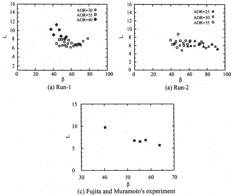
Fig. 6 Plot of dimensionless wave length versus the aspect ratio.
