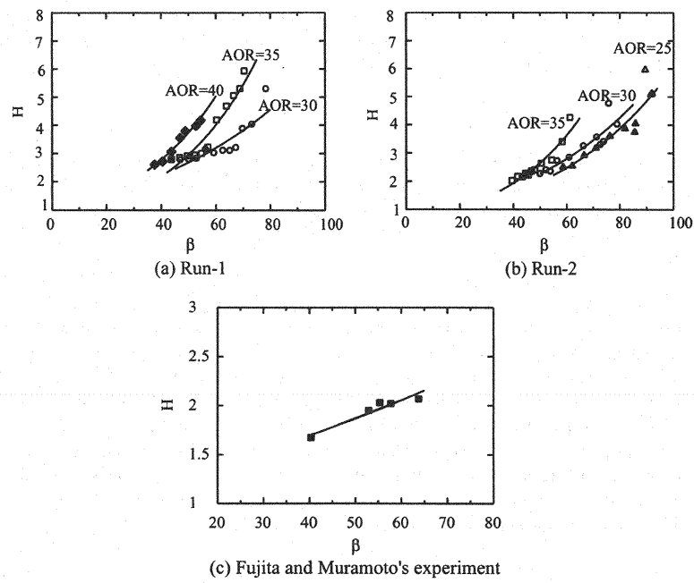
Fig. 4 Plot of dimensionless bar migration speed versus the aspect ratio.
