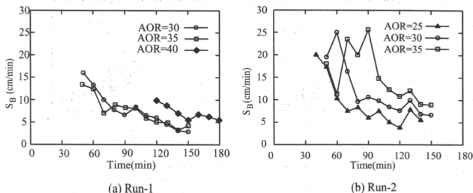
Fig. 3 Plot of the bar migration speed versus bank strength. AOR stands for the critical angle of repose.
