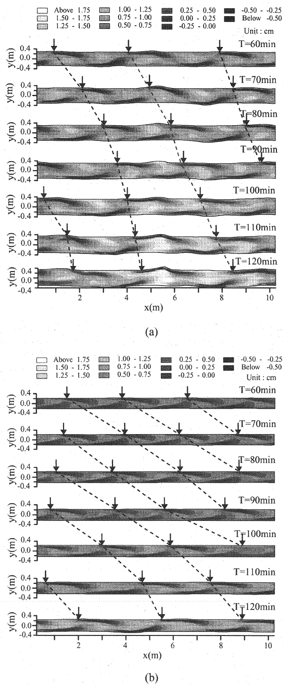
Fig. 2 Bar migration in the channel with the angle of repose : (a) 25 deg.; (b) 35 deg. for Run-2, respectively. The arrow symbol indicates the bar front in the left bank, and the dashed line indicates the bar migration along the bank with time. Flow is left to right.
