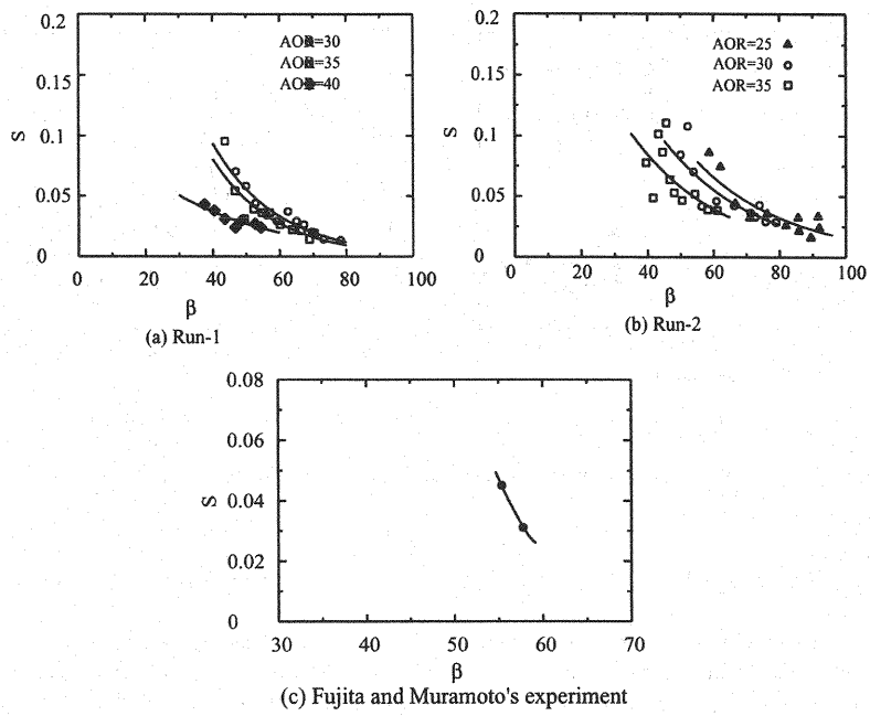
Fig. 4 Plot of dimensionless bar migration speed versus the aspect ratio.
