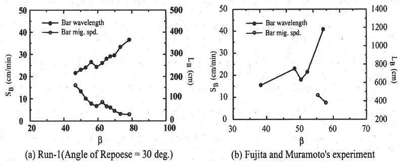
Fig. 7 Plot of the bar migration speed and wavelength versus the aspect ratio.
