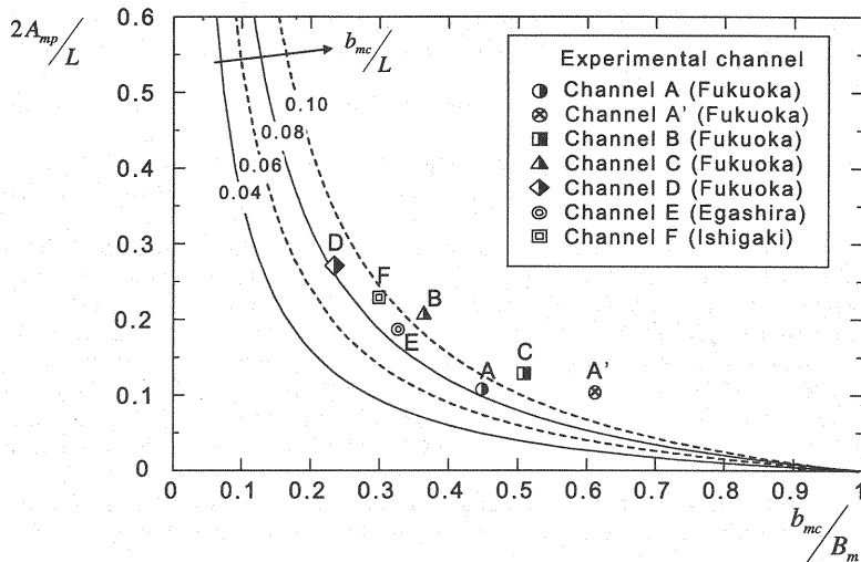
Figure 6 Non-dimensional plan shape parameters of experimental channels
