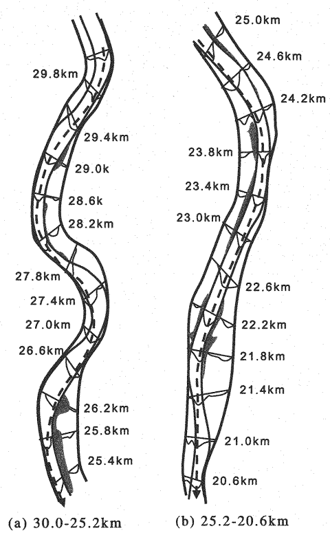
Figure 10 Surface velocity distribution and maximum velocity filament at Gono River in July 1983 flood (analyzed by using aero photograph)
