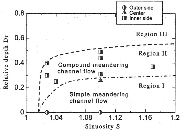
Figure 8 Flow classification diagram based on location of the maximum velocity at meander apex section (Experimental channel)
