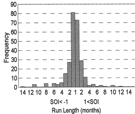
Fig. 11 Histogram of duration analysis result for the case in which the absolute value of SOI is more than 1
