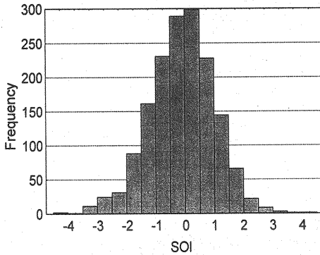
Fig. 7 Histogram of original SOI time series
