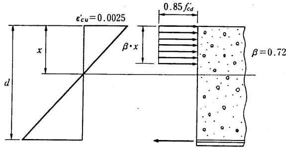
Fig. 9.2 Equivalent Stress Block
