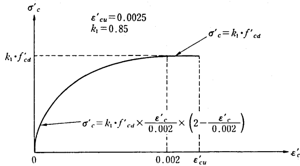
Fig. 9.1 Modeled Stress-Strain Curve of Concrete
