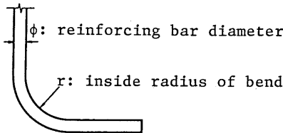
Commentary Fig. 4.3.1—Inside bending radius.
