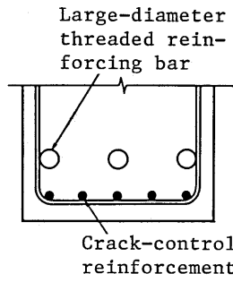
Commentary Fig. 3.3.1—Method of arranging crack-control reinforcement.
