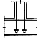
Commentary Fig. 4.4.5—Threaded reinforcing bar anchorage at end of main reinforcement of column and wall.
