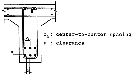
Fig. 4.2.1—Clearances between reinforcing bars and center-to-center spacing.
