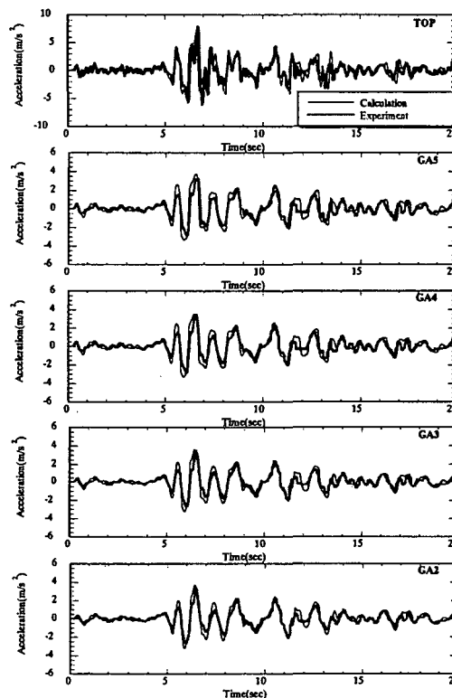
Figure 8 Time history of the acceleration in the case of Single pile II
