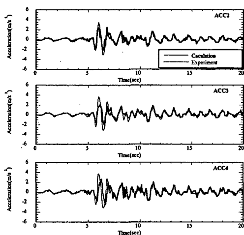
Figure 5 Time history of acceleration of Ground II
