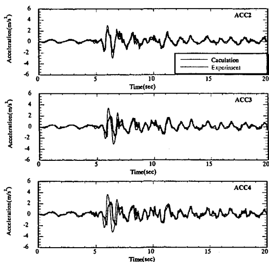
Figure 4 Time history of acceleration of Ground I
