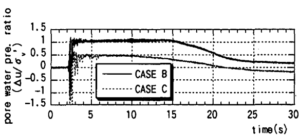
図－8 過剰間隙水圧比 (GL-0.2m)
