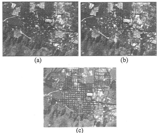
Fig. 6. Enhanced image of Nueva San Salvador. (a) Enhanced pre-event image. (b) Enhanced post-image and location of the landslide. (c) GIS map overlaid on the satellite-enhanced image.
