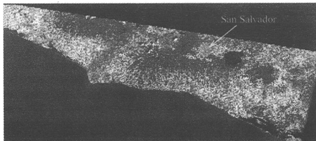
Fig. 2. Post event image (RGB 752) of Landsat 7
