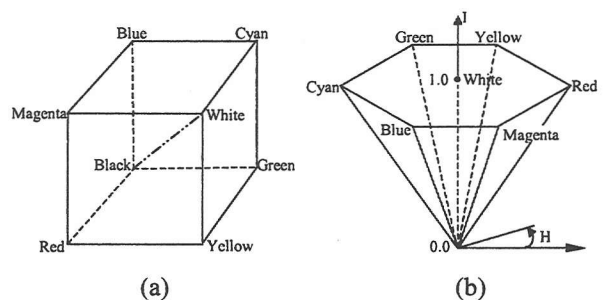
Fig. 3. The color space. (a) Red-green-blue color cube. (b) Hue-saturation-intensity hexcone.
