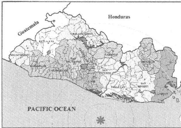
Fig. 1. Map of the Republic of El Salvador and the location of the epicenter.
