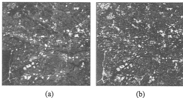
Fig. 5. San Salvador city. (a) RGB (321) composite color image. (b) Sharpened image by HSI transformation and merged with the panchromatic band.
