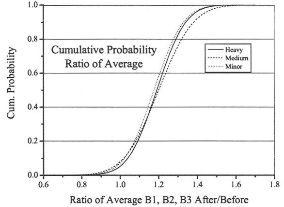
Fig. 9. Cumulative probability of the ratio after/before of the averaged images.
