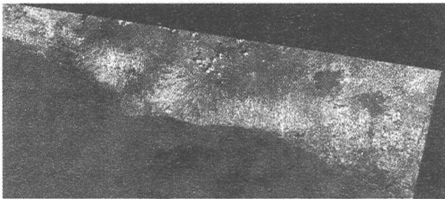
Fig. 8. Ratio after/before of the average of the first three visible bands.
