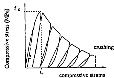
Fig. 3 Stress-strain model for concrete in compression
