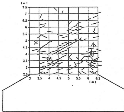
Fig. 6 Resultant crack pattern in the final stage
