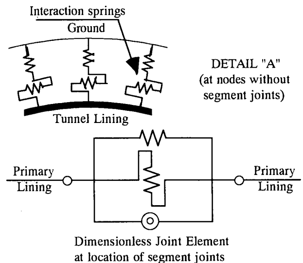
Fig.1 Tunnel-Ground system
