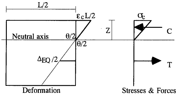
Fig. 3 Model for determining the flexural stiffness
