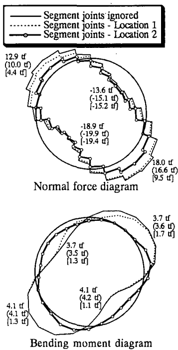
Fig.9 Response of Karimojima tunnel
