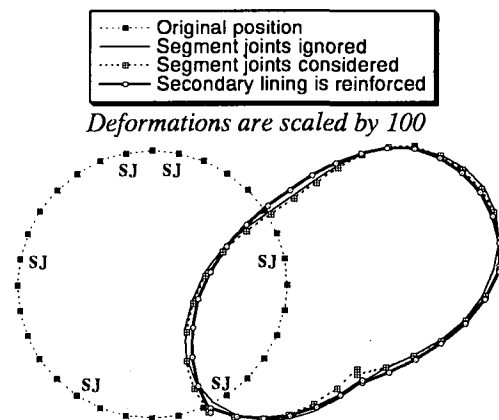
Fig.12 Deformation of Takamatsu tunnel
