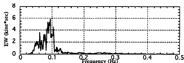
Fig. 4 Fourier Spectrum of Hokkaido Toho Oki Earthquake at Akashi Station.
