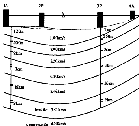
Fig. 2 The Crustal Structure under the Akashi Kaikyo Bridge.
