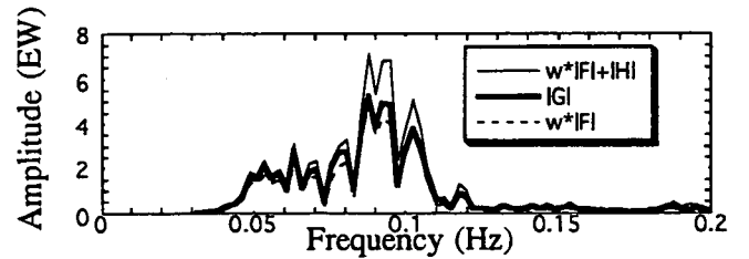
Fig. 7 Fourier Amplitude Spectra of No.55 Record at Akashi Station
