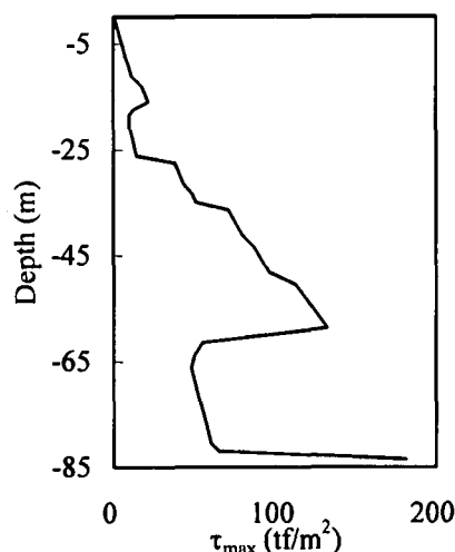
Fig.3.2 Identified maximum shear stresses
