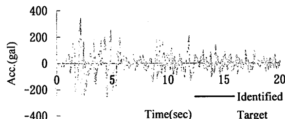
Fig.5.3 Identified input acceleration
