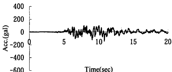
Fig.6.2 Calculated downward wave at basement (F)
