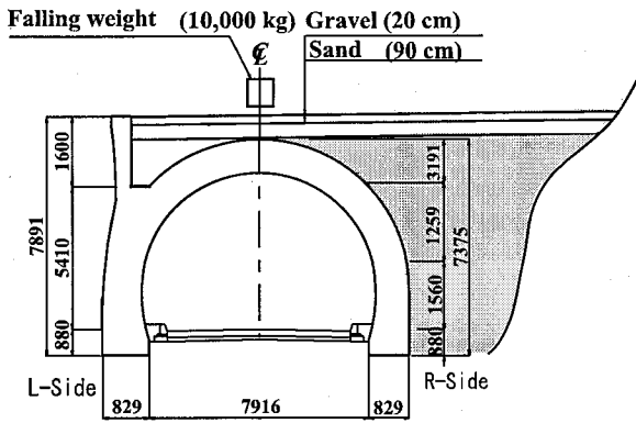
(a) Absorbing system with sand cushion
