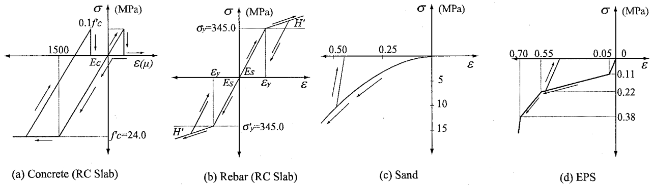
Figure 4 Stress strain relationships of material constitutive models
