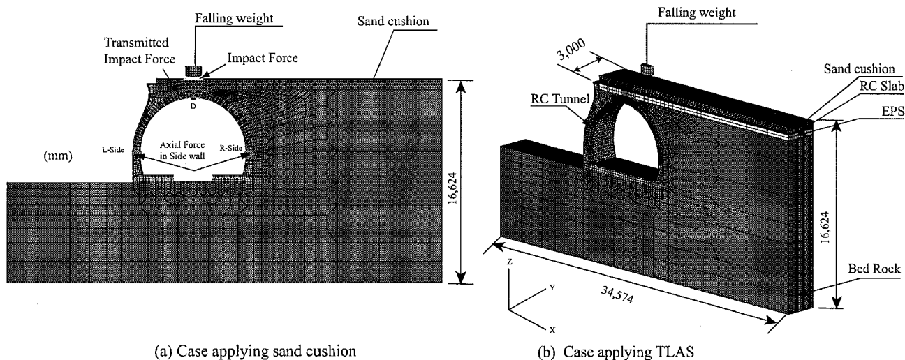
Figure 2 FE mesh model in cases applying two absorbing system
