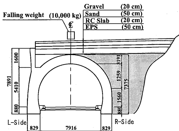
(b) Three layer absorbing system
