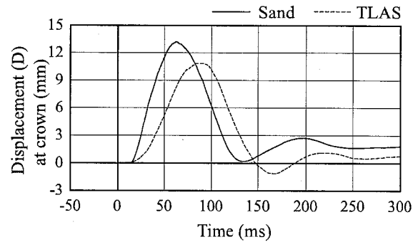
Figure 6 Displacement ( D ) at crown of tunnel
