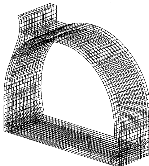
Figure 3 Rebar arrangement of tunnel
