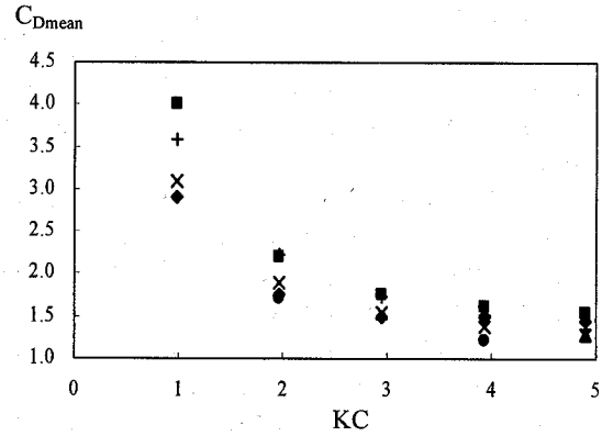
Fig.3 C_{D\text{mean}} : ■Anagnostopoulos and Minear 10) ; ◆Lin et al. 13) ; ▲Obasaju et al. 12) ; •Bearman et al. 14) ; Present Results (×Oscillatory Flow; +Oscillating Body).
