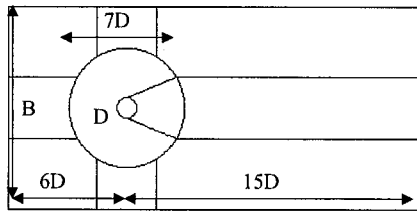
Fig.2 Computational Domain.
