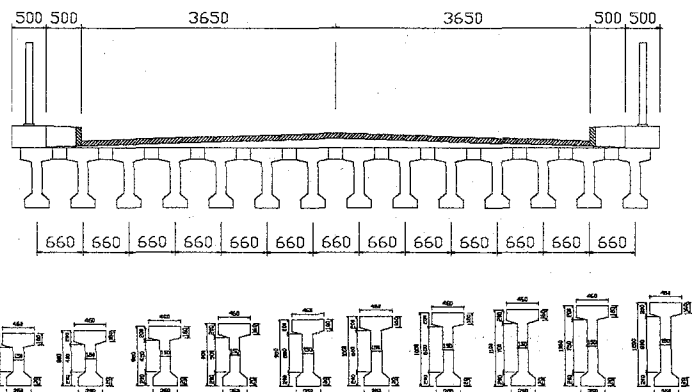
Fig2. Bridge with 14 girders
