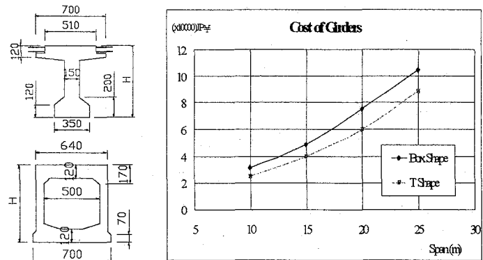
Fig1. Shape of section
