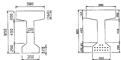
Fig4. Section of selected girders
