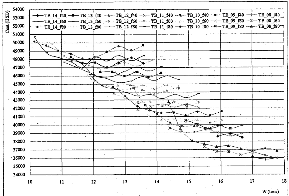
Fig3. The total cost of bridge super structures
