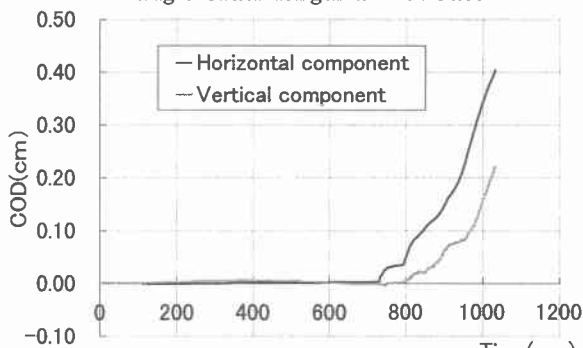
Fig.7 COD at notch(Case2/4)
