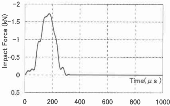
Fig.3 Impact force for analysis
