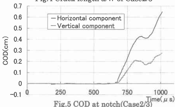
Fig.5 COD at notch(Case2/3)
