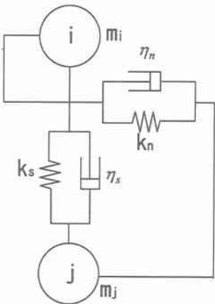
Fig.1 Springs and particles of DEM
