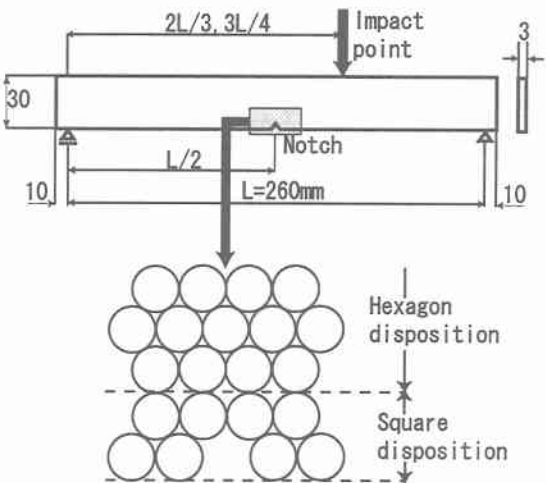
Fig.2 Analytical model
