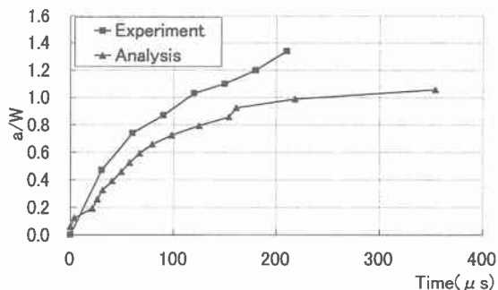
Fig.4 Crack length a/W of Case2/3
