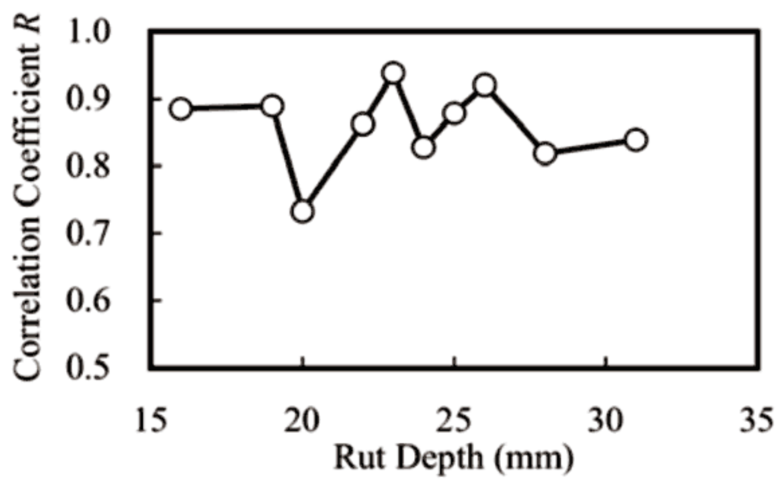
(a) Correlation Coefficient Between QFM and Measurement
