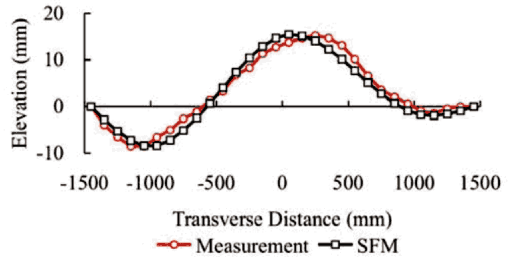
(b) SFM ( R=0.98 , L=220m )
