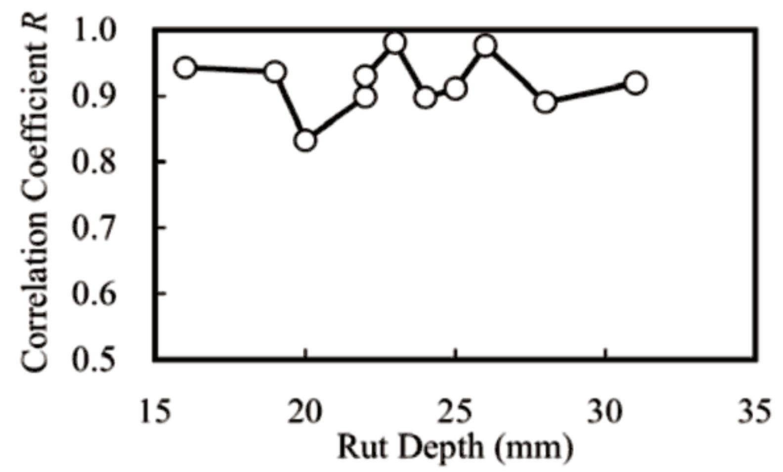
(b) Correlation Coefficient Between SFM and Measurement
