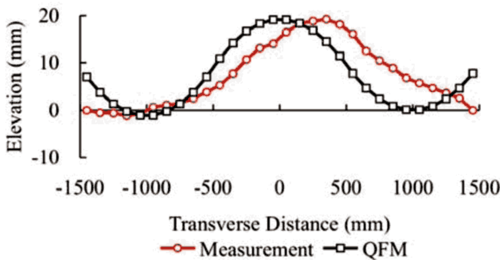
(a) QFM ( R=0.73 , L=240m )
