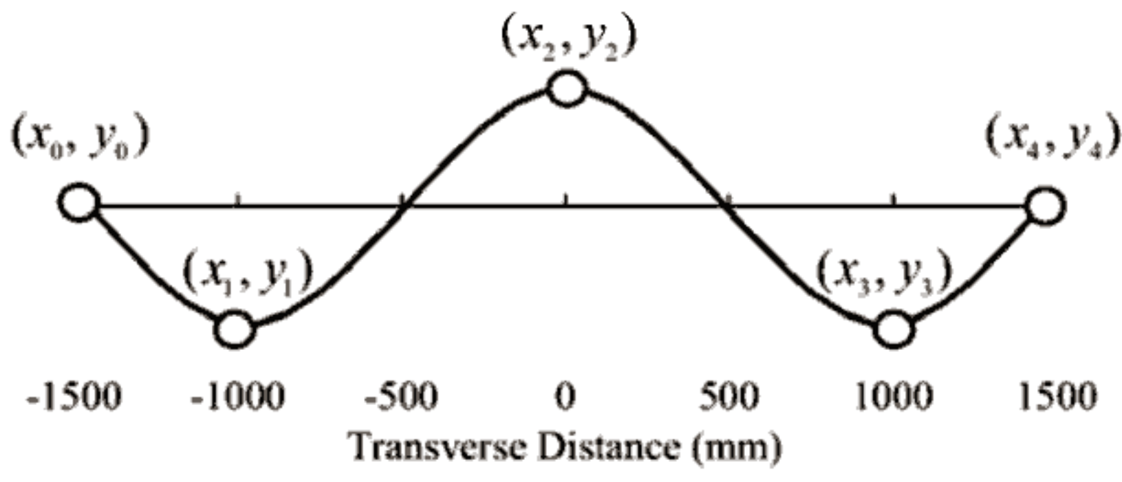
Fig.6 Designed by Cubic Spline
