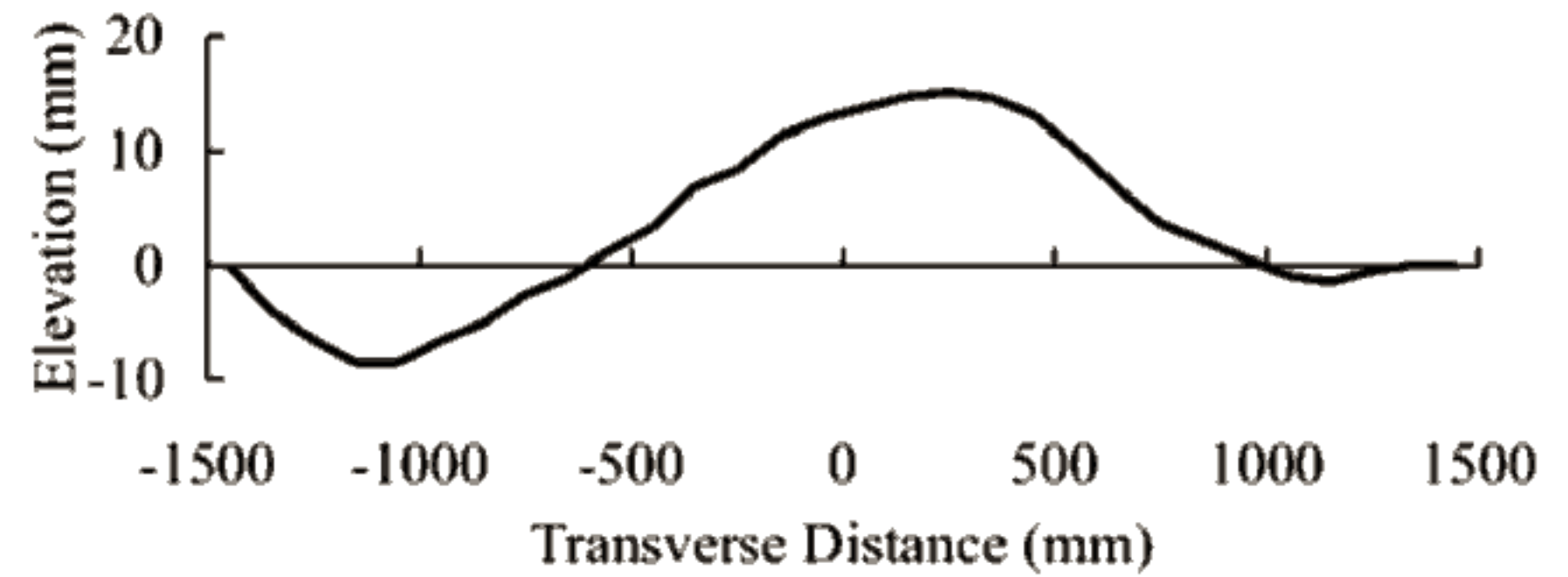
Fig.1 An Example of Transverse Profile
