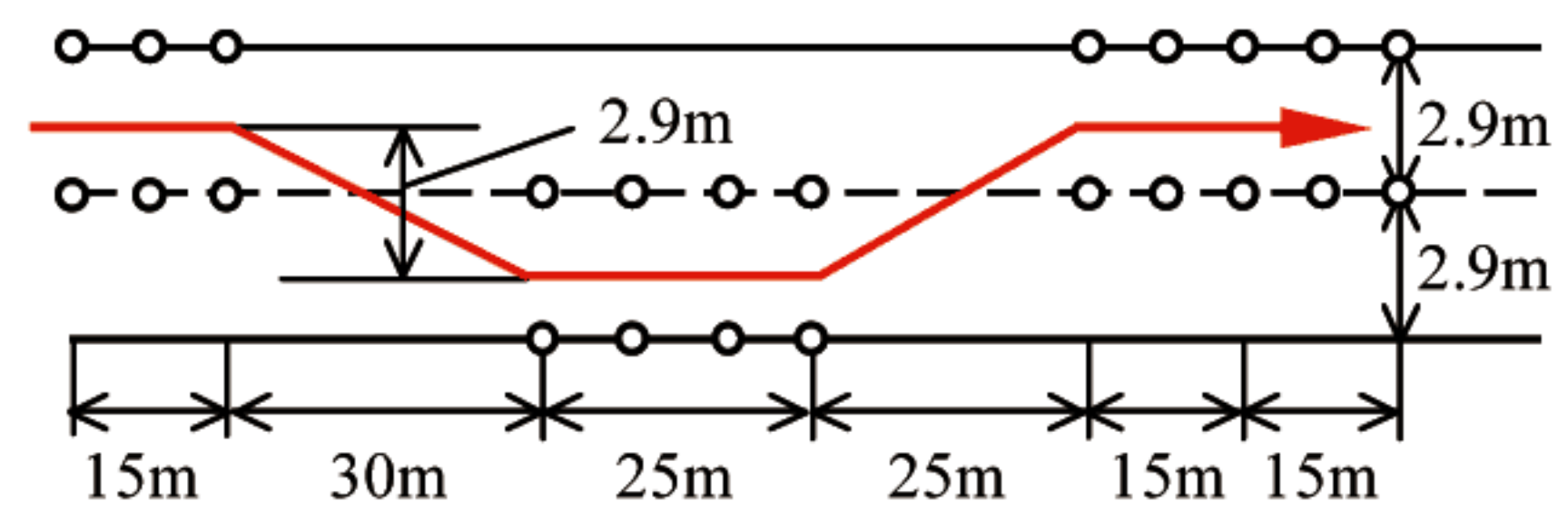
Fig.14 Double Lane-Change Track
