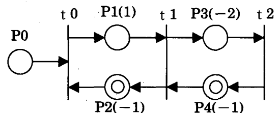
Fig.5 Combined Net of Vehicle's Arrival and Progress
