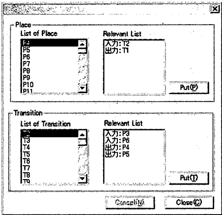
Fig.7 Interface for “Layout Places and Transitions”
