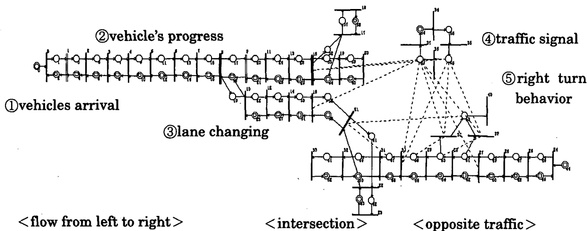
Fig.1 Petri-net Representation of Traffic Flows around Signalized Intersection
