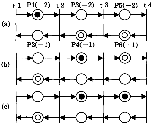
Fig.2 Basic Sub Net of Vehicle's Progress
