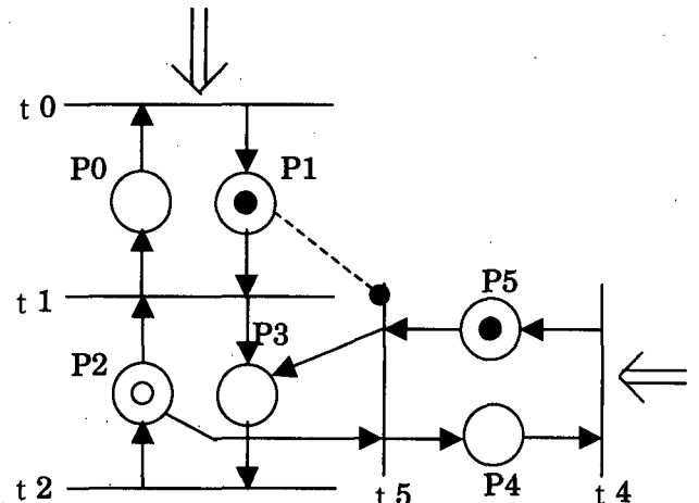
Fig.4 Priority Setting by Inhibitor Arc
