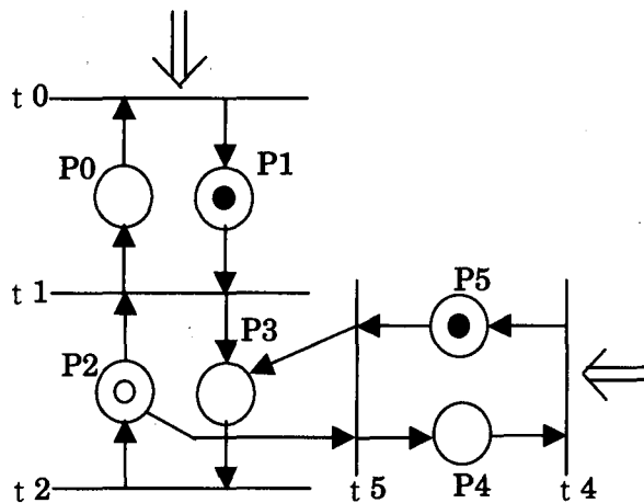
Fig.3 Conflict State in Traffic Petri-nets
