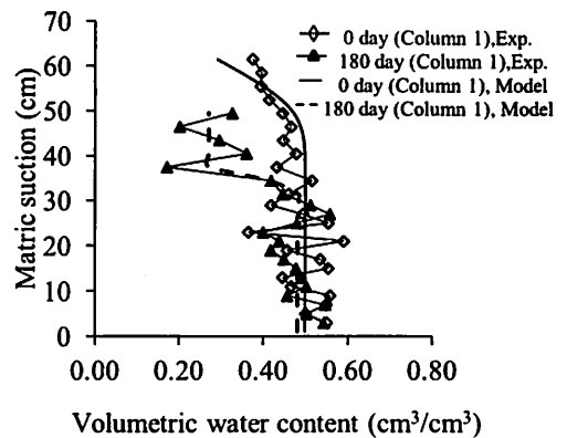
Fig. 4 Temporal dynamics in water retention curve in simulated landfill.
