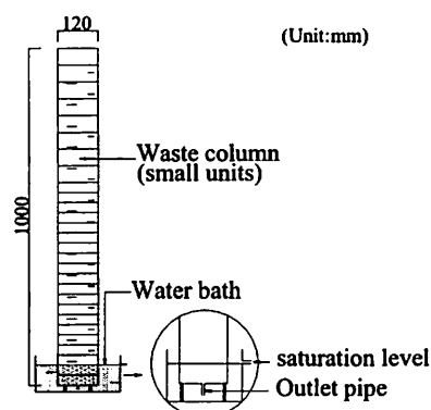
Fig. 1 Schematic diagram of the experimental column.
