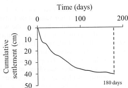
Fig. 2 Cumulative settlement variation in Column 2.
