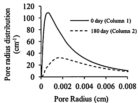
Fig. 5 Derived pore size distribution of simulated landfill.
