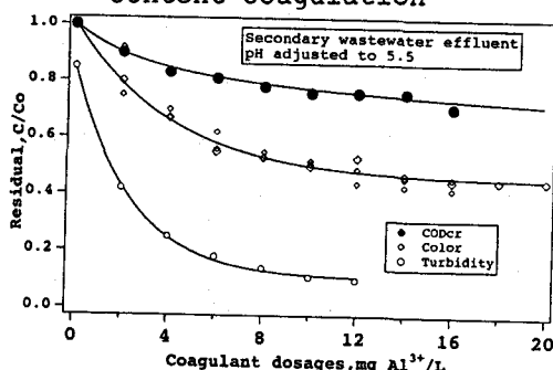
Fig 3: Effect of coagulant dosages on the removal of effluent content
