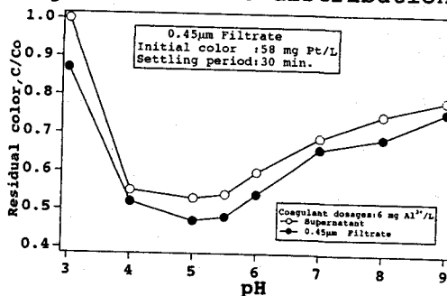
Fig 5: Effect of pH on color coagulation
