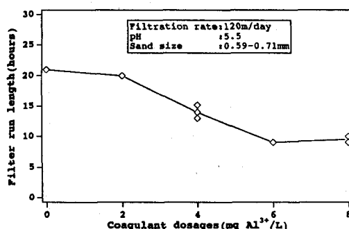
Fig 12: Variation of the filter run length with the coagulant dosages
