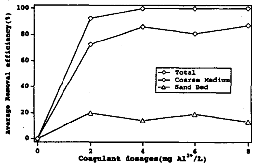
Fig 10: Effect of coagulant dosages on color flocs removal efficiency
