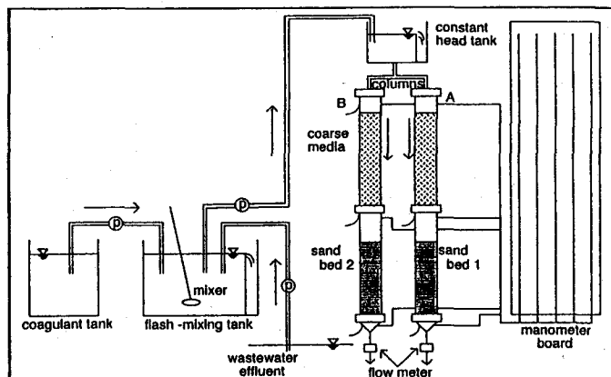
Fig1: Experimental Apparatus
