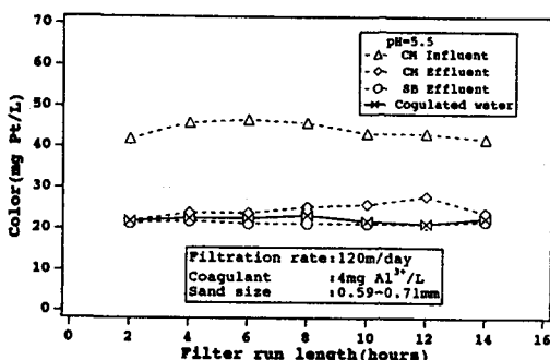
Fig 7-b: Variation of the color during the filtration with pH control
