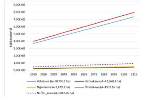
Fig.3 Impacted Sub-basin Avg Soil Loss estimated
