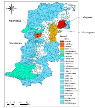
Fig.2 Sub-basin soil loss Impact Map of Study area
