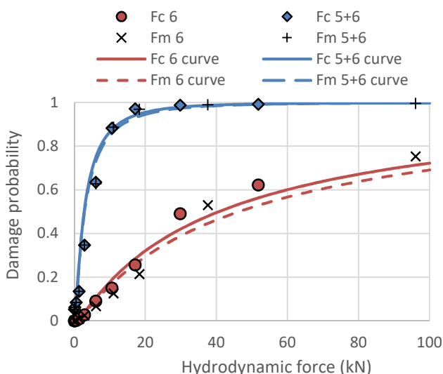
Fig. 2 Fragility functions ( F_c and F_m as explanatory parameters)
