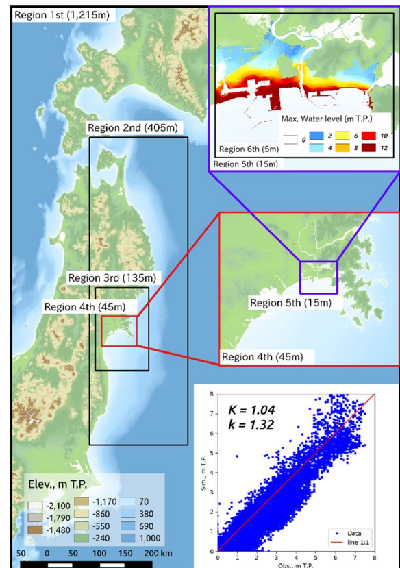
Fig. 1 Study area, simulation results and model verification
