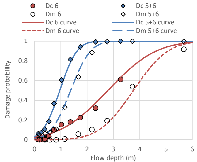
Fig. 3 Fragility functions ( D_c and D_m as explanatory parameters)
