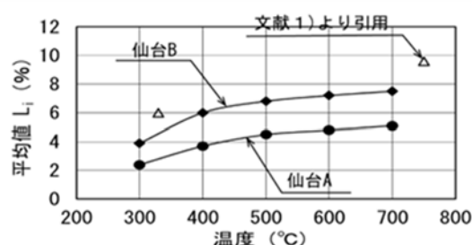
図-1 強熱減量試験
