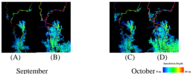
Fig.4 Temporal and spatial variation of inundation area (A and C : 250m resolution and B and D : 1km resolution)
