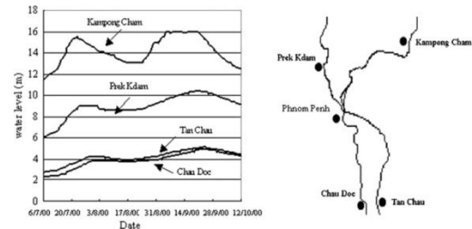
Fig.2 Water levels for boundary conditions
