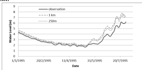
Fig 3 Comparison of calculated and observed water level at Phnom Penh
