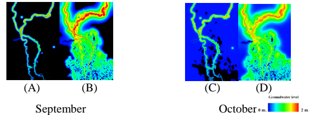
Fig.5 Temporal and spatial variation of groundwater level (A and C : 250m resolution and B and D : 1km resolution)
