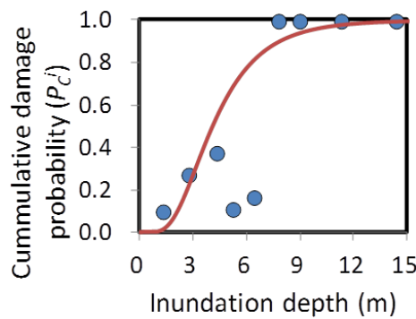
Figure 2. Damage probability curve of pedestrian bridge during the 2011 tsunami
