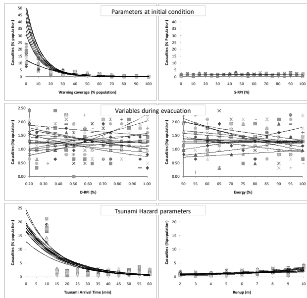
Figure 3 Output scatter plots
