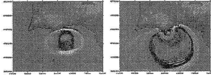
Fig. 3: Tsunami's propagation at 600 s and 1200 s after the generation.
