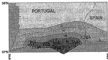
Fig. 1: Ground shake intensity from the 1722 earthquake.
