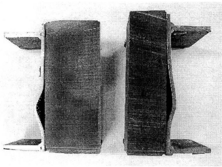
(a) Narrower plate (b) Wider plate Photo 1 Buckling deformation and Epoxy(S/E-UX, UY)
