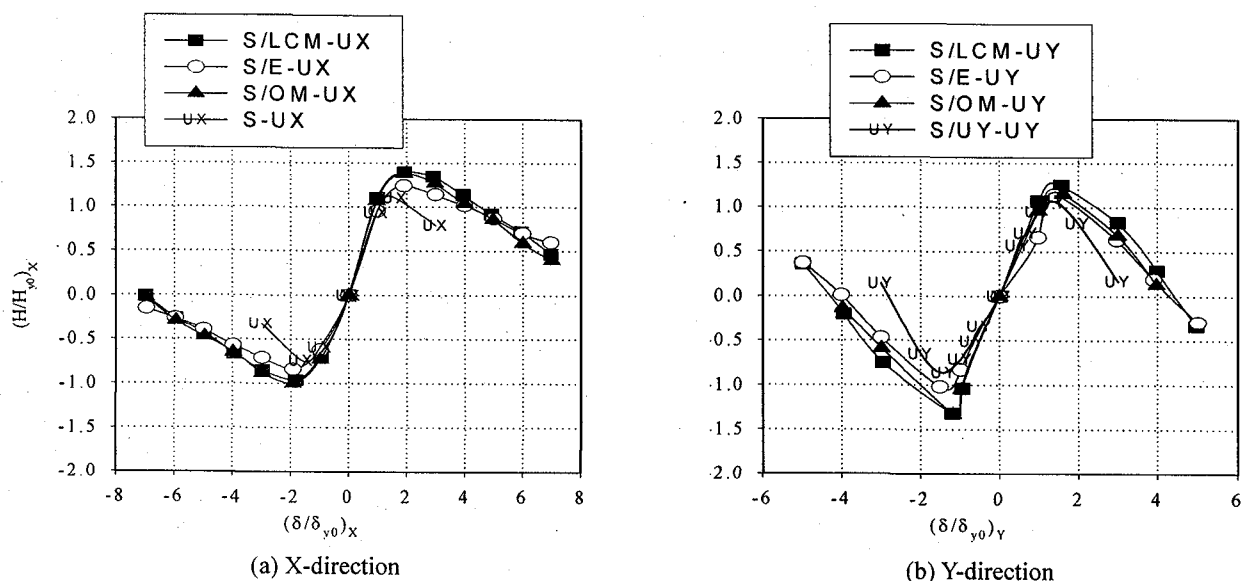
Fig. 8 Envelop curves
