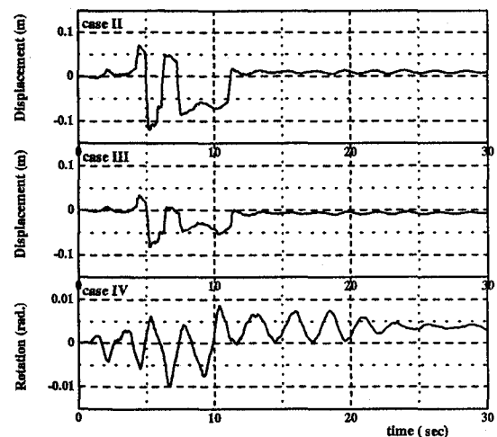
Fig. 7 Displacement time history of high stiffness energy dissipation device system ( K/K_0 = 0.10 )
