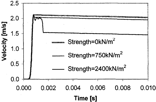
Fig.10 Fly-off velocity of crown depending on strength of interface
