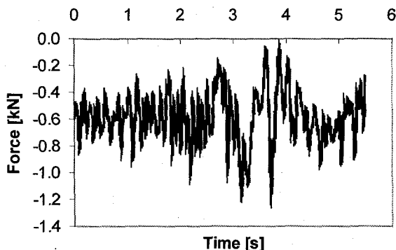
Fig.6 Force at the column-crown interface
