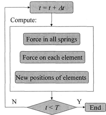
Fig.4 Solution algorithm
