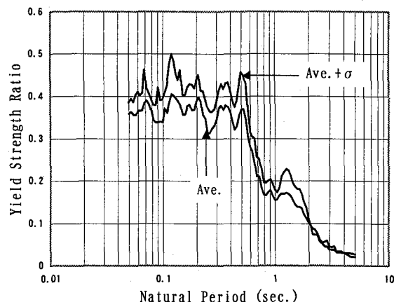
Figure 12 Strength demand spectra of ground motions with average and average+ \sigma damage potential in 50 years at Rio Dell
