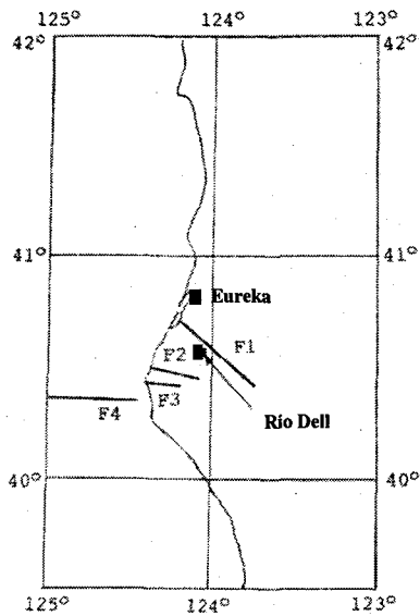
Figure 5 Map of fault model around Eureka and Rio Dell
