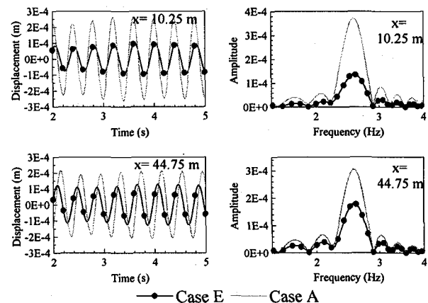
Fig. 13 Response time histories and Fourier amplitudes. (continue)
