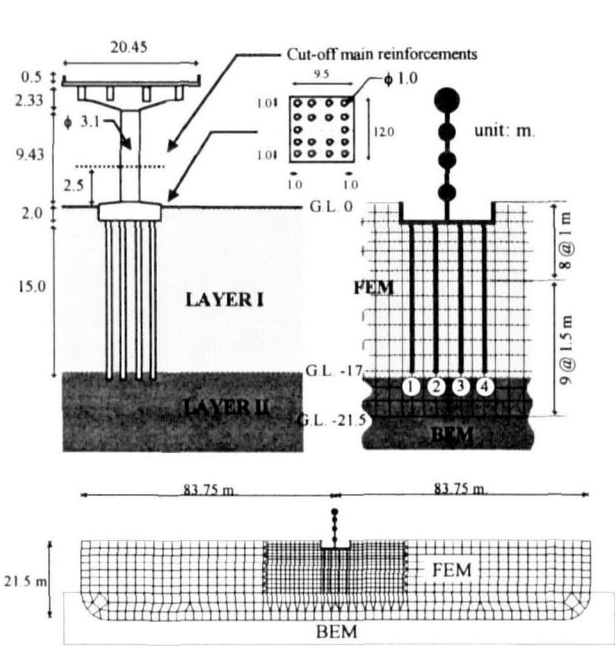
Fig.1 Typical bridge of the Japanese Highway network and its model of analysis.
