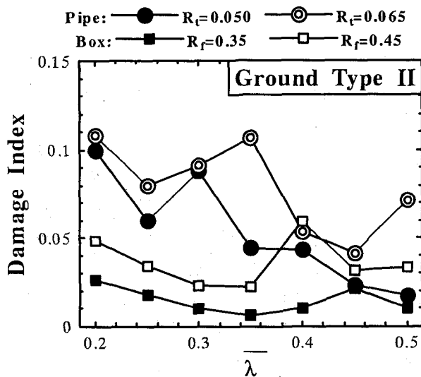
(a) Under Level 2 • Type I accelerograms
