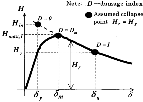
Fig. 1 Degradation of strength (monotonic loading)
