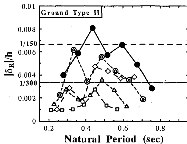
(c) cross section: R_t = 0.050 , t = 23mm (SM490)
