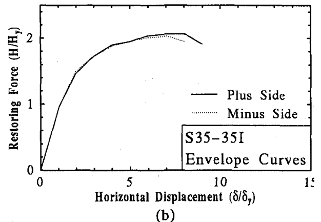
Fig. 3 Cyclic Test Result of Specimen S35-35I
