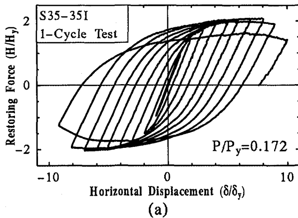
Fig. 3 Cyclic Test Result of Specimen S35-35I
