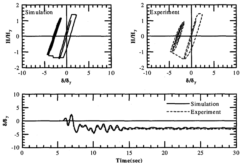
Fig.11 Response of TS11-30-11 to 1.5 \times \text{HKB} accelerogram
