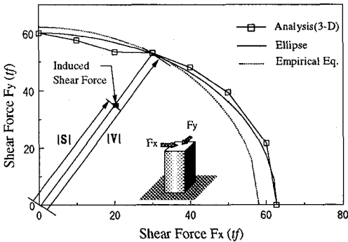
Figure 6 Shear Capacity of Member subjected to Multi-Directional Forces
