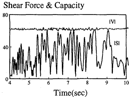
Figure 7 Norm of Shear Force (ISI) & Capacity (IVI) in C3
