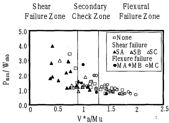
Figure 3 Failure Condition
