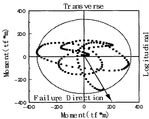
Figure 13 Interaction Diagram of Moment & Failure Envelop Curve
