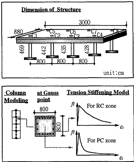
Figure 5 Structural Modeling
