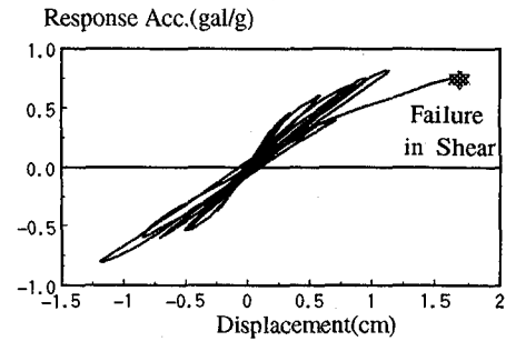
Figure 10 Hysteric Curve of Response Acceleration and Displacement
