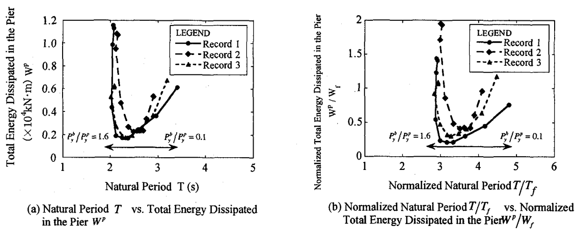
Fig. 14 Dependence of Total Energy Dissipated in the Pier on the Natural Period (Device with Positive Post-Yield Stiffness)
