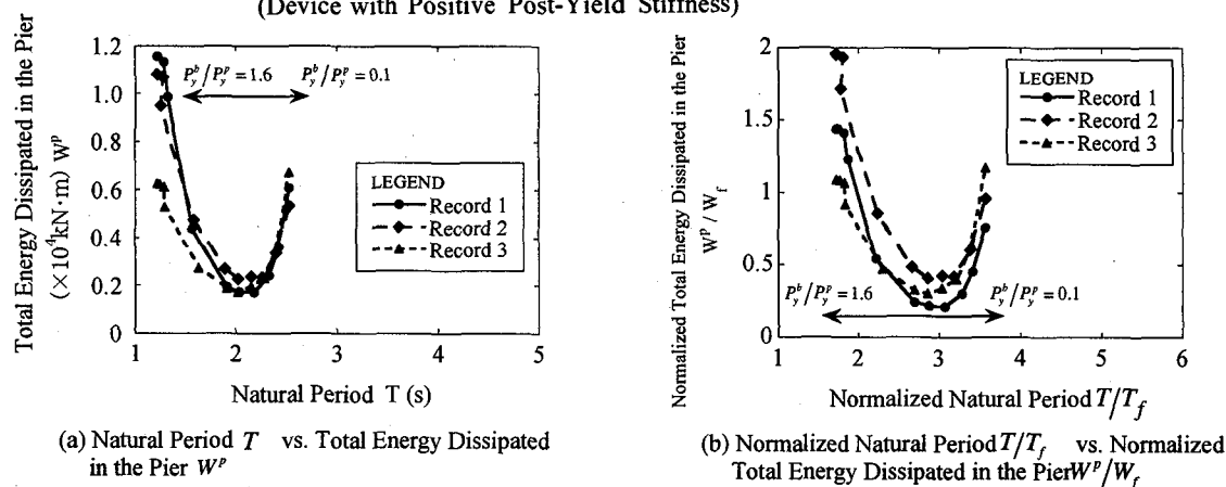
Fig. 15 Dependence of Total Energy Dissipated in the Pier on the Natural Period computed with use of Cracked Stiffness of the Pier (Device with Positive Post-Yield Stiffness)
