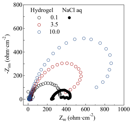
Fig. 3 Nyquist plots (1:5).
