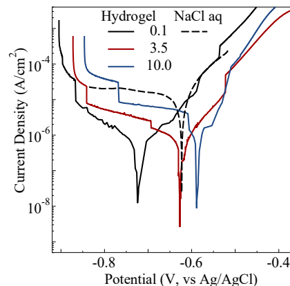
Fig. 6 Polarization curves (1:10).
