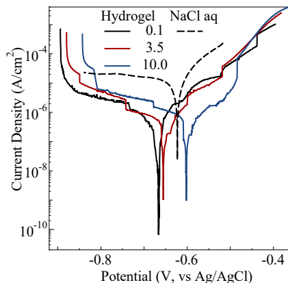
Fig. 5 Polarization curves (1:5).
