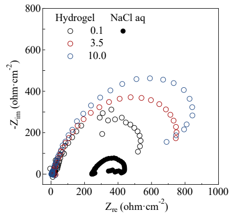
Fig. 4 Nyquist plots (1:10).
