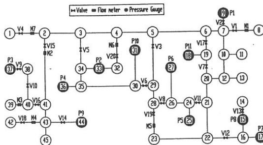
Fig. 1. Block 12 of the Fukuoka City water supply
