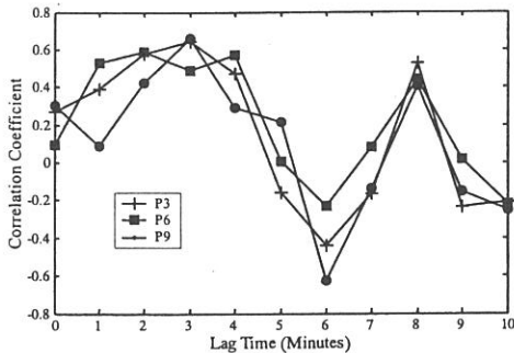
Fig. 3. Cross-correlation between electrically motor valve (V9) and selective pressure gauges.
