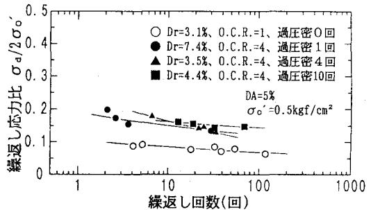
図-4(A) 繰返し回数～繰返し応力比関係
