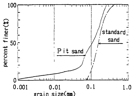
Fig. 1 Grain size distribution of samples
