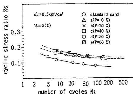
Fig. 2 Stress ratio versus number of cycles to liquefaction
