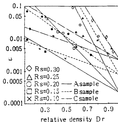
Fig.5 gradient of constant uplift \varepsilon versus relative density D_r
