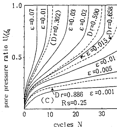
Fig.4 group of model pore pressure curves with examples of test results
