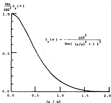
Fig.3 Graphical Representation of Spectral Density
