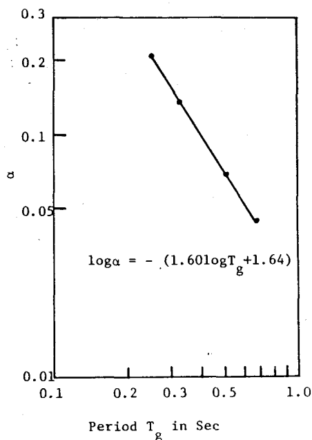
Fig.2 Relationship between the Parameter \alpha and the Predominant Period of the Ground
