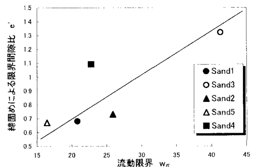
図-6 液状化限界間隙比と流動限界の関係
