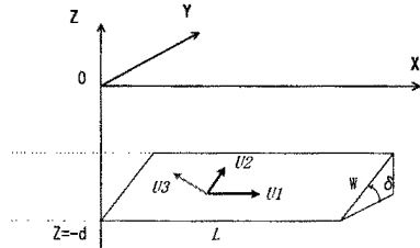
図-2 Source Model
