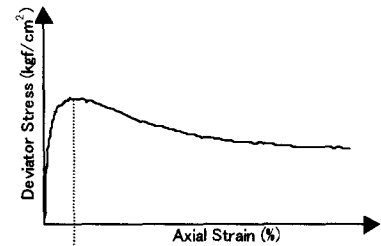
Fig. 3 Stress-Strain Curve
