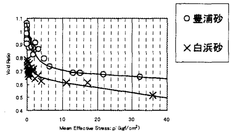
Fig. 5 Steady-State Line
