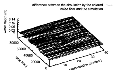
Fig. 3 absolute difference between simulation and colored-filter model
