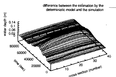
Fig. 2 absolute difference between simulation and deterministic model
