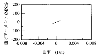
(c) 免震支承
