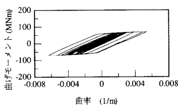
(a) 鋼製支承
