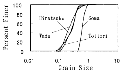
Fig. 1 Grain Size Distribution
