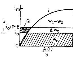
Fig.1: The distribution of tension water capacity in the basin (simplified xinanjiang model)
