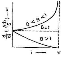
Fig.2: Density function of the simplified xinanjiang model
